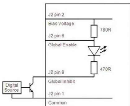
Global Inhibit using System Signal
