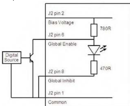
Global Enable using System Signal
