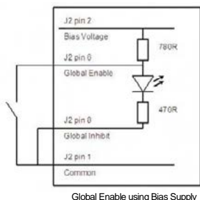
Global Enable using Bias Supply
