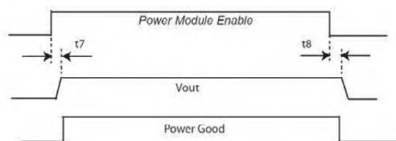
Power Module power good signal
