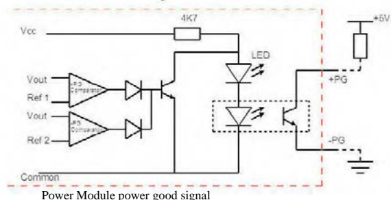
Power Module power good signal
