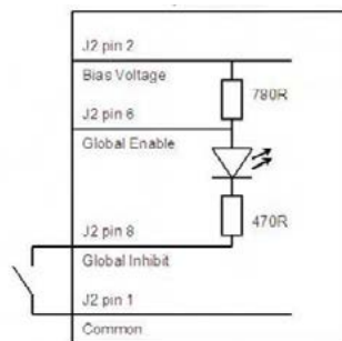
Global Inhibit using the Bias Supply
